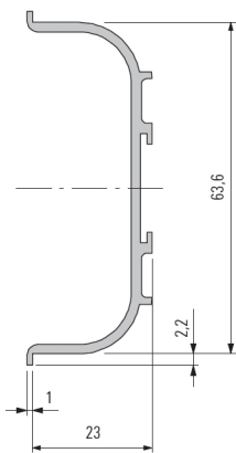
U-formos profilis (6 m) art.901013
